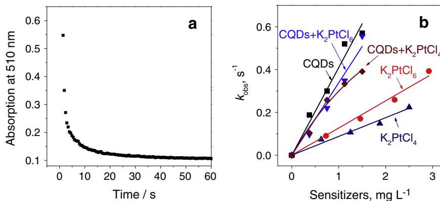
Fig. 7. (a) Decay time profiles of absorption at 510 nm due to QuPh + -NA in the electron transfer from QuPh + -NA to CQDs in a mixed solution (2.0 mL) of a deaerated aqueous buffer (pH 7.0) and MeCN [1:1 (v/v)]. QuPh + -NA was produced by photoirradiation of QuPh + -NA (0.44 mM) in the presence of NADH (1.0 mM). (b) Plots of the pseudo-first-order rate constants ( k_{\text{obs}} ) for electron transfer from QuPh + -NA vs weight concentrations (CQDs, K 2 PtCl 6 and K 2 PtCl 4 ).
