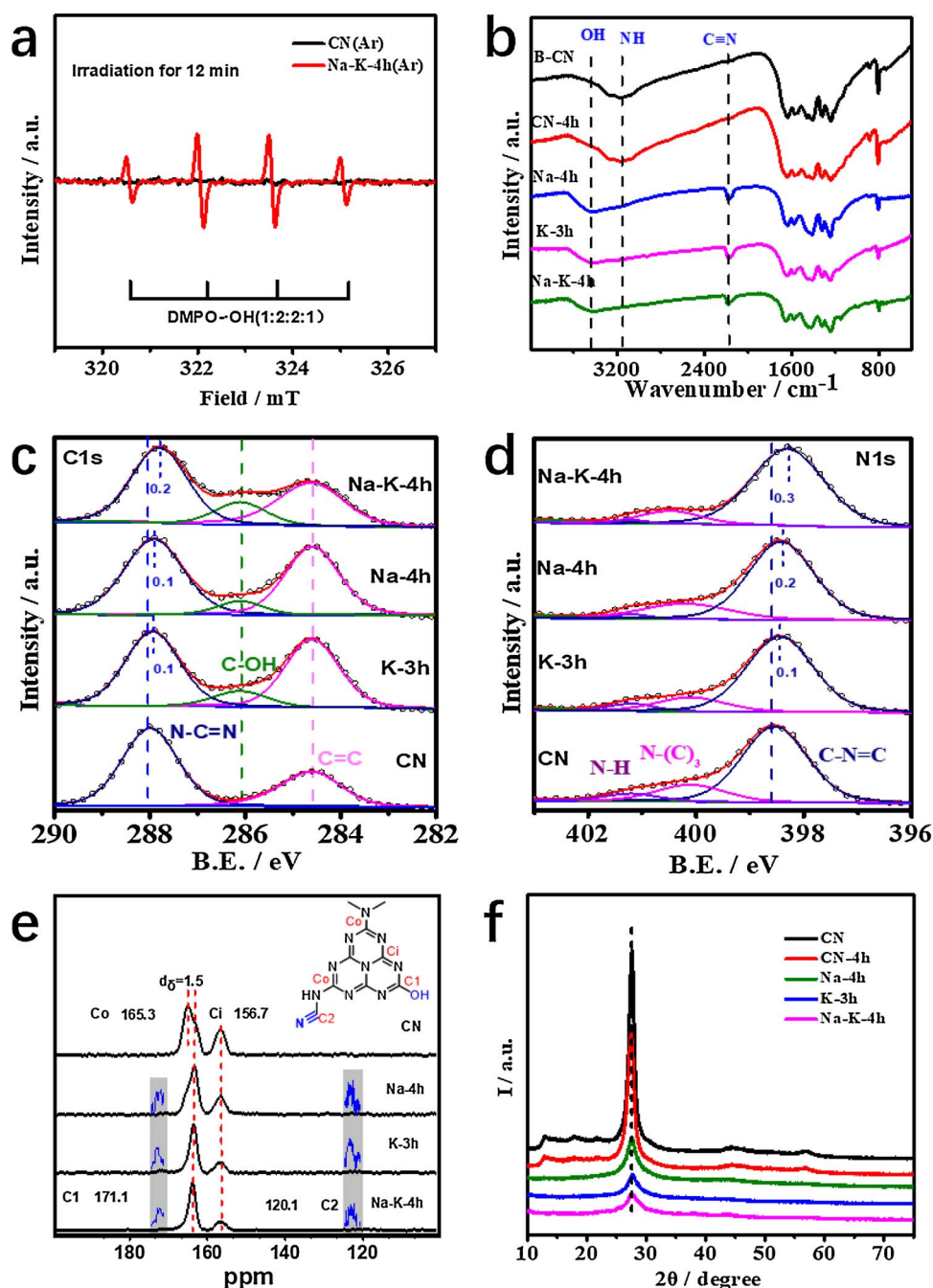
Fig. 3. (a) ESR signal of Na-K-4h and CN under visible-light irradiation for 12 min Ar atmosphere. (b) FT-IR spectra of samples. The high resolution spectra of C1s (c) and N1s (d) of samples, (e) Solid-state 13 C MAS NMR spectra of these samples and proposed structure diagram (inside), the amplified spectra could be seen in Fig. S10. (f) XRD spectra of samples.
